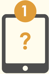
Authentication Challenge
