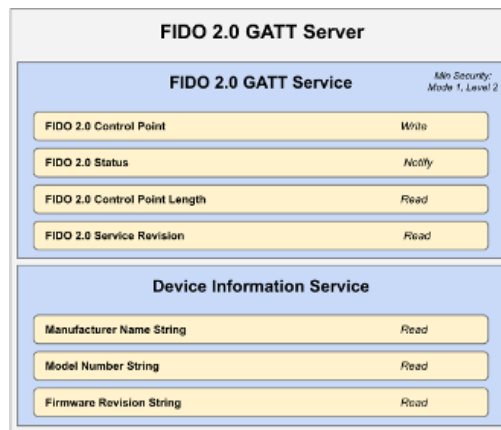
Figure 6 Mandatory GATT services and characteristics that MUST be offered by a FIDO Authenticator. Note that the Generic Access Profile Service ( BTGAS ) is not present as it is already mandatory for any Bluetooth Low Energy Technology compliant device.
