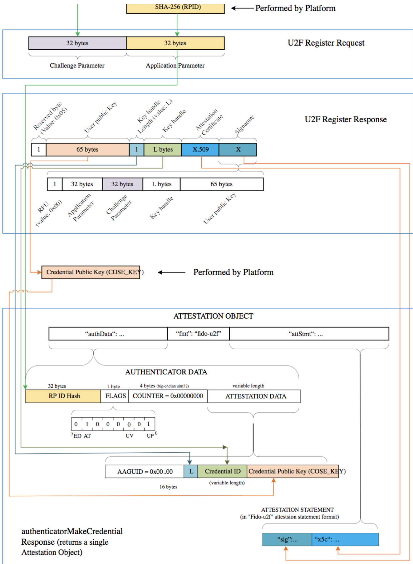
Figure 2 Mapping: WebAuthn authenticatorMakeCredential to and from CTAP1/U2F Registration Messages.
