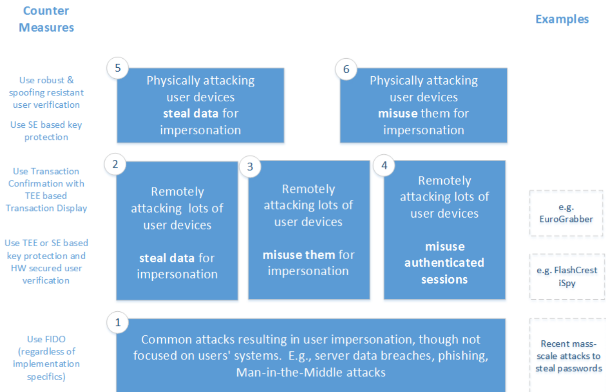
Fig. 2 Attack Classes
