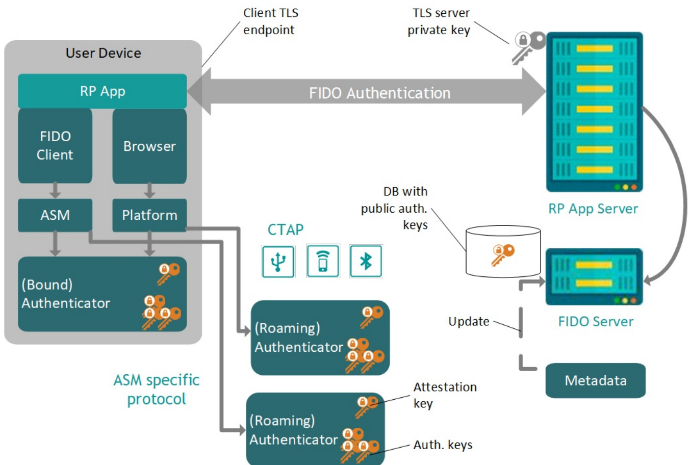
Fig. 1 FIDO Reference Architecture
