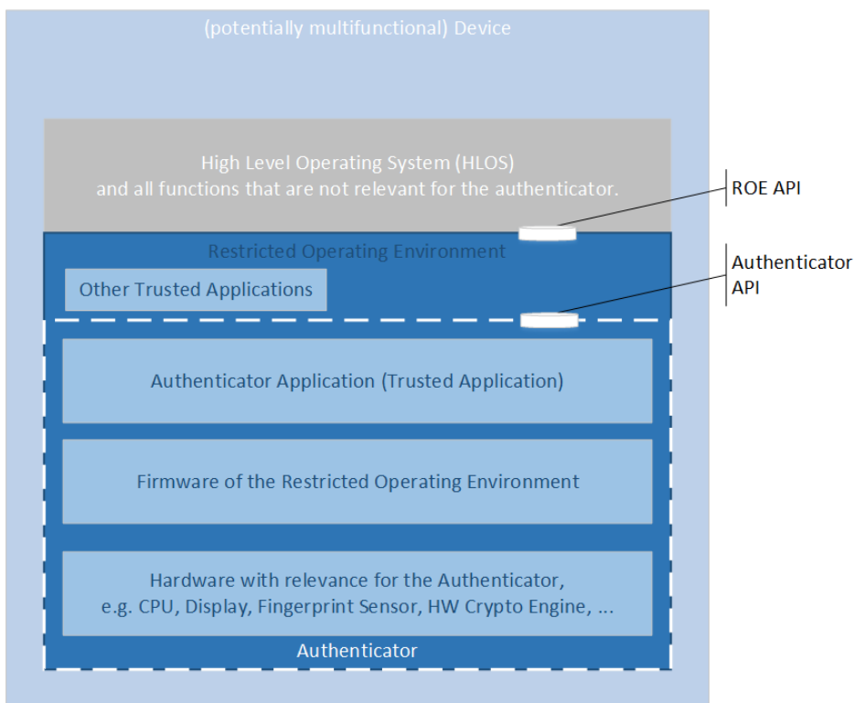
Fig. 3 Restricted Operating Environments Architectural Overview
