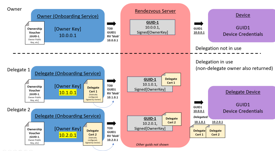
Figure 7 Rendezvous for Owner versus Delegates
