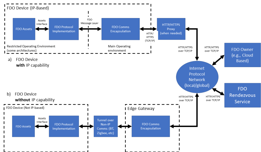
Figure 1 FIDO Device Onboard Transport Interfaces
