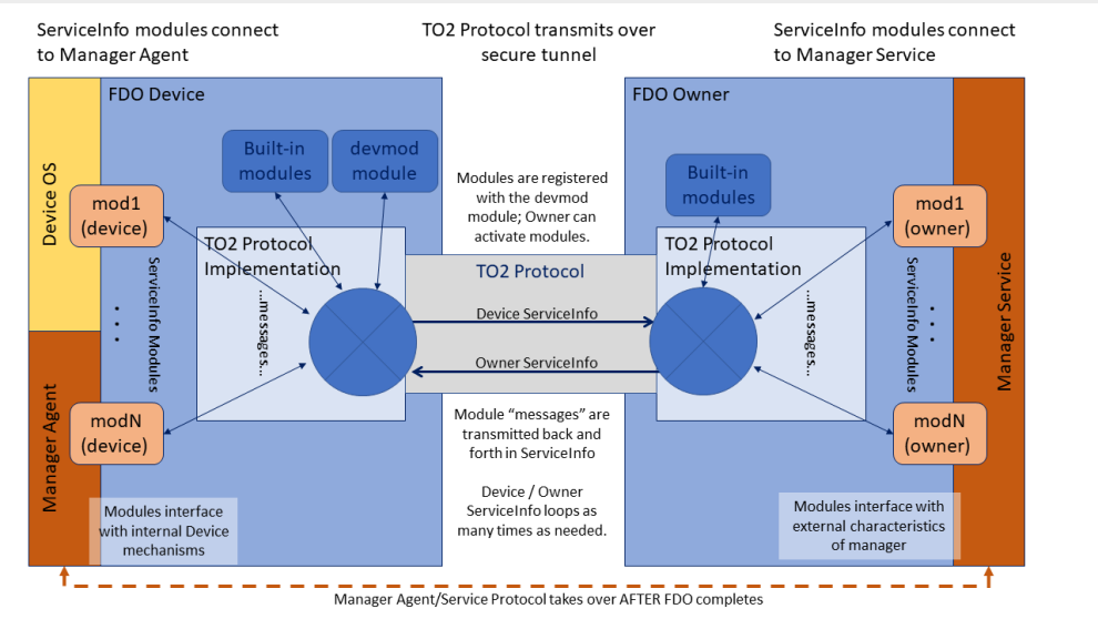
Figure 9 Management Service - Agent Interactions via ServiceInfo End of informative comment
