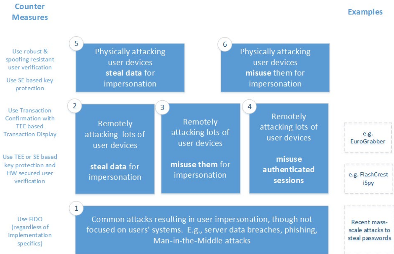
Fig. 2 Attack Classes
